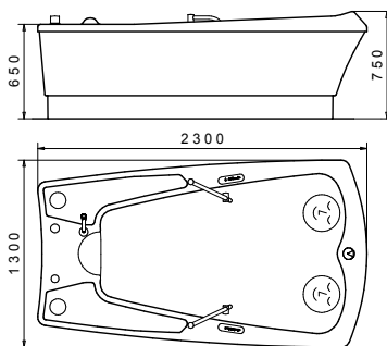
Maße California Twin
